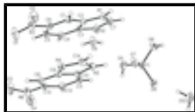
Fig. 1. The molecular structure of the title compound, with the atomic numbering scheme. Displacement ellipsoids are drawn at the 30% probability level. H atoms are shown as small spheres of arbitrary radius.
