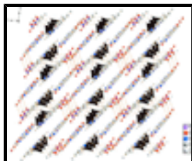
Fig. 3. A packing diagram for the title compound, viewed along the a axis. Dashed lines indicate hydrogen bonds.
